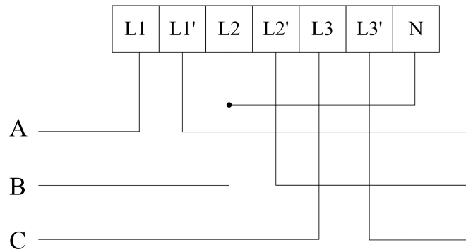
Fig 7 Three phase three lines direct connect
