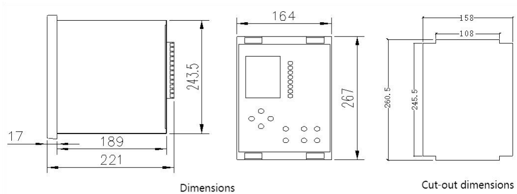
Figure 4.1 Dimensions and cut-out dimensions
