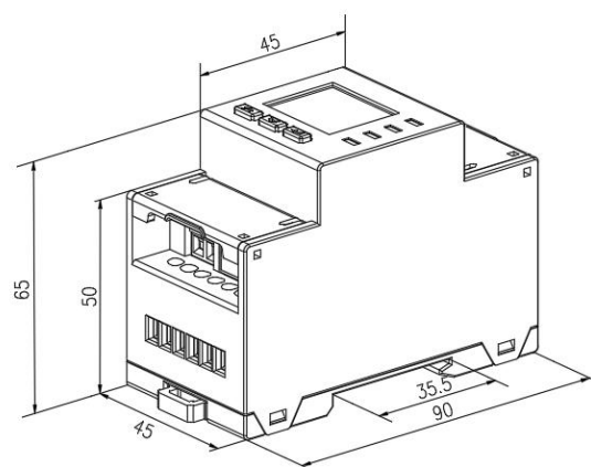
图 2 ADL400N-CT Figure 2 ADL400N-CT
