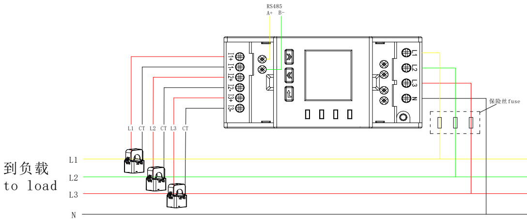
图 4 ADL400N-CT 三相四线经互感器接入 Figure 4 ADL400N-CT Three-phase Four-wire Connection Through Current Transformer
